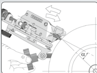
The Clearance angle is set by tilting the base...
